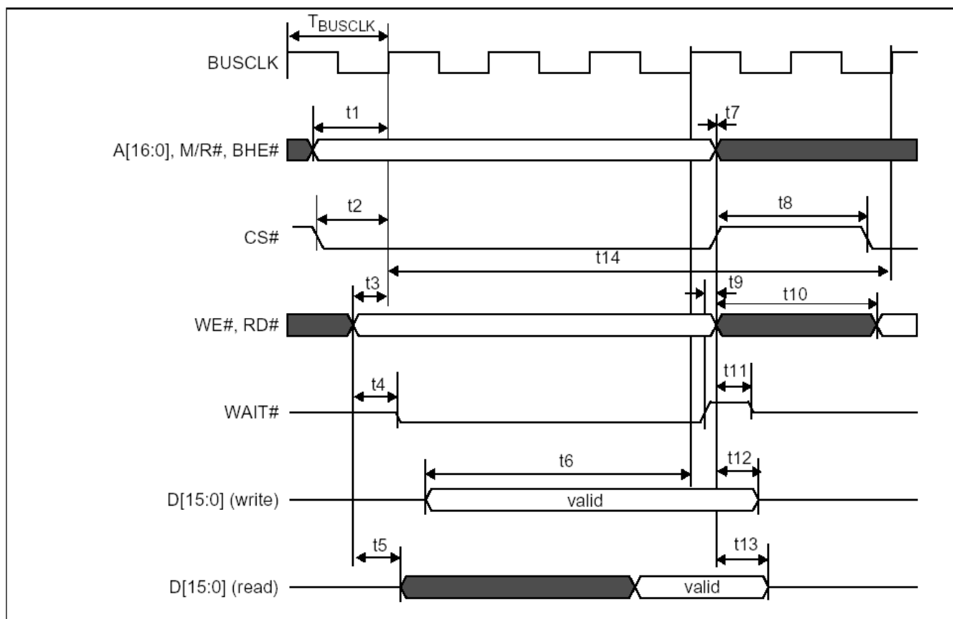
6-1. Interface Timing
