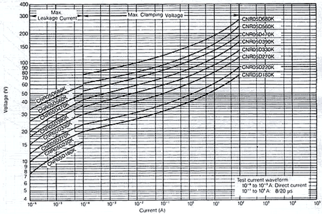
V-I Curve (CNR05D180K to CNR05D680K)
