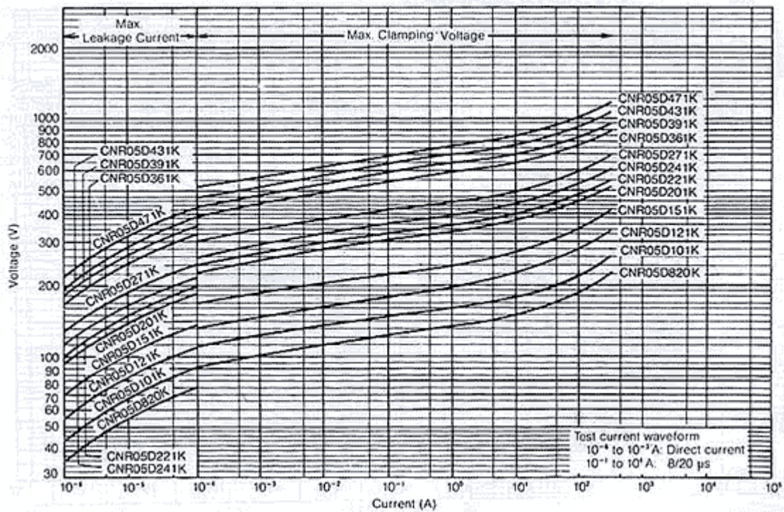
V-I Curve (CNR05D820K to CNR05D471K)
