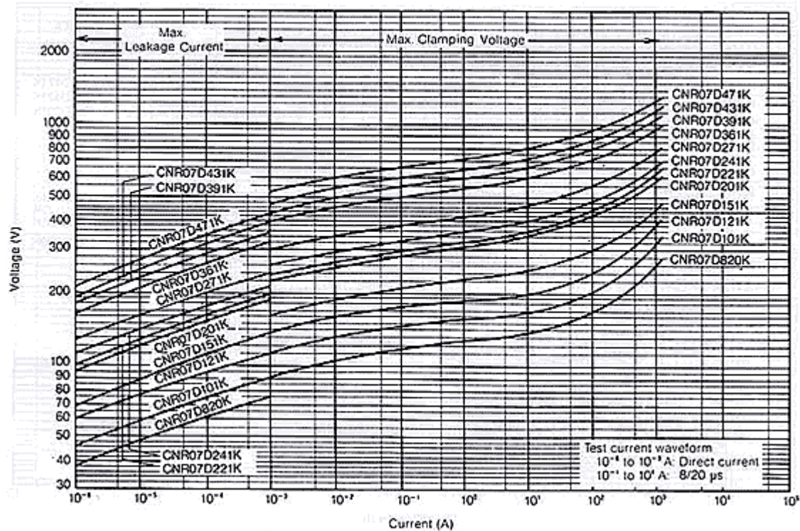
V-I Curve (CNR07D820K to CNR07D471K)
