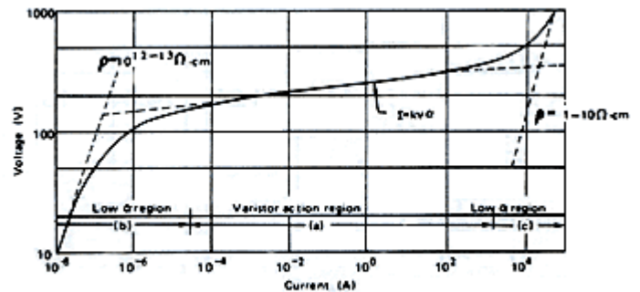
Typical Varistor V - I Curve
