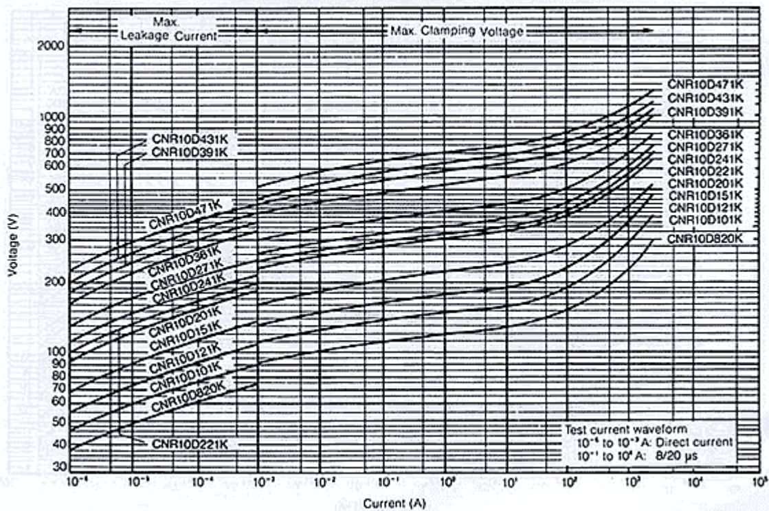
V-I Curve (CNR10D820K to CNR10D471K)
